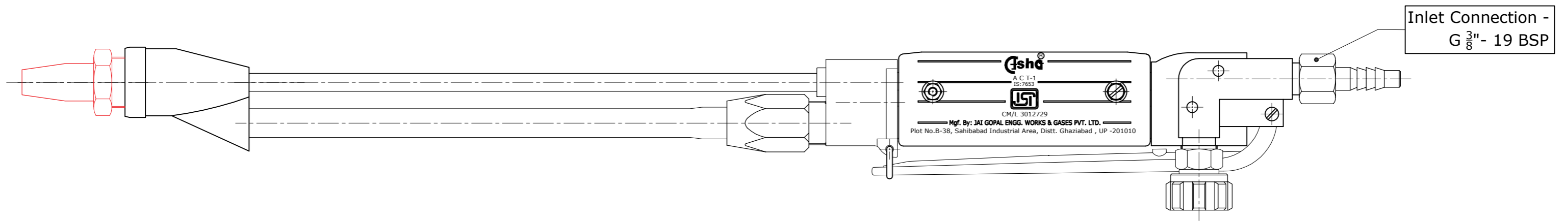
CUTTING TORCH WITH HEAD 180°
